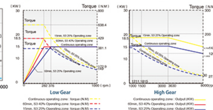
BT-50 Gear head (1:4.23)
