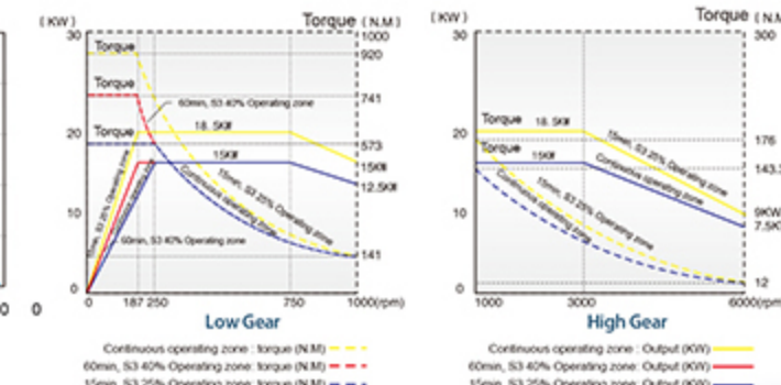
BT-50 Gear head (1:4.23)
